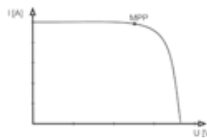
Schematic view of IV characteristic Voltage value at MMP
